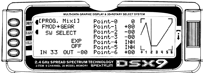
Flight Mode switch in ST1 position
