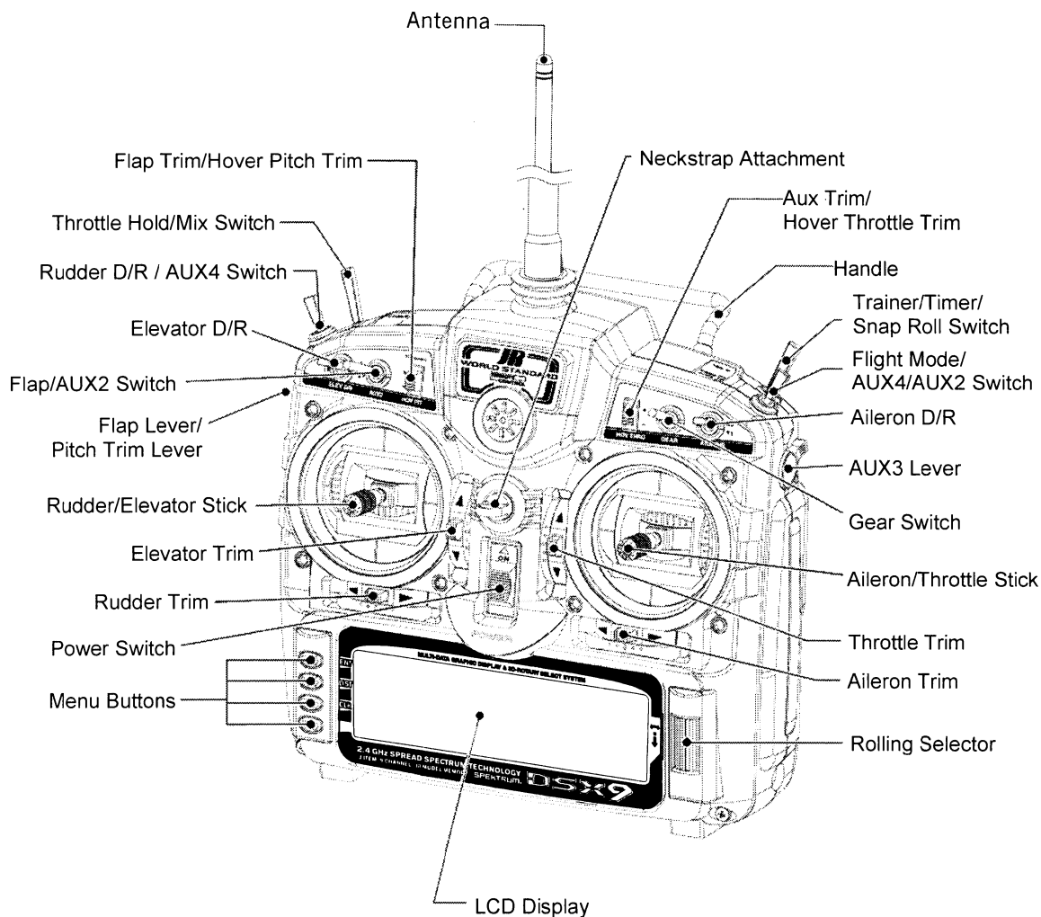
Transmitter shown with stick mode 1 selected
